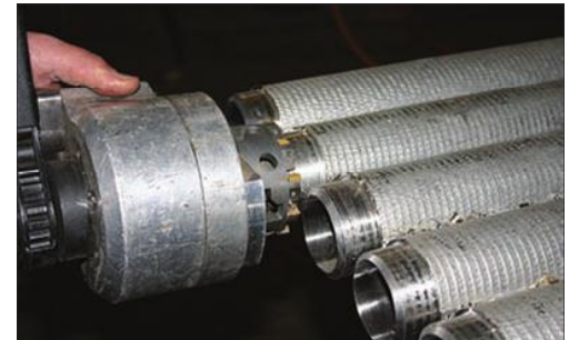
Low RPM and extraordinary torque at the cutting bit make the Mini Millhog a great choice for many tube stub and overlay removal applications.
