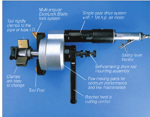
Titanium nitride coated cutter blades provide smooth milling, without cutting oils, and produce a clean continuous chip.
