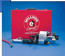
Esco MILLHOG® "Mini" Series end prep tools rigidly mount to the pipe or tube I.D. by a draw rod clamping assembly which centers the tool automatically to produce a clean bevel with a square end.
